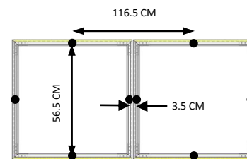
Position of the U hangers
