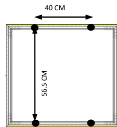
Position of the L hangers
